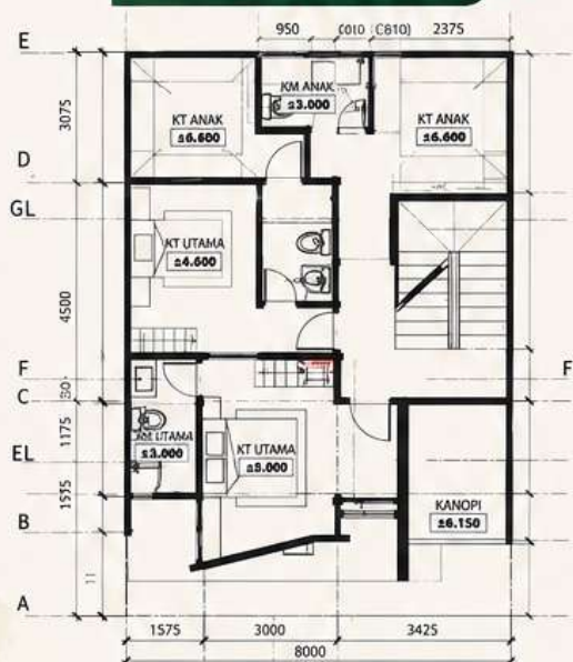
DENAH LANTAI 3
