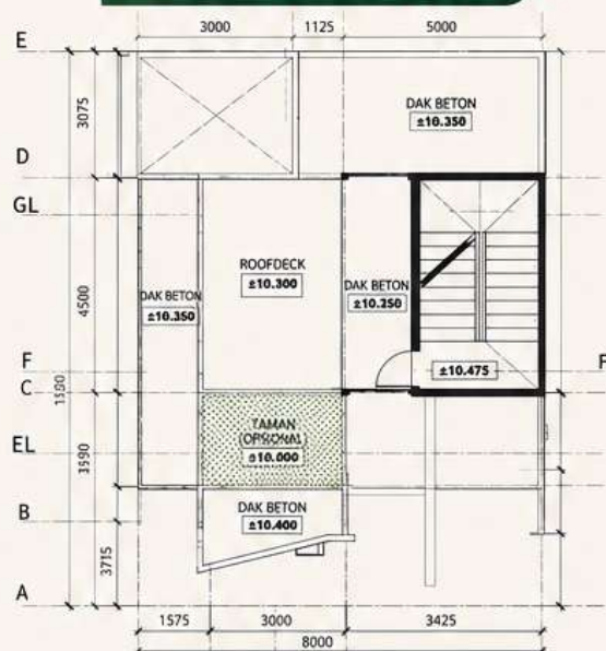
DENAH LANTAI ATAP
